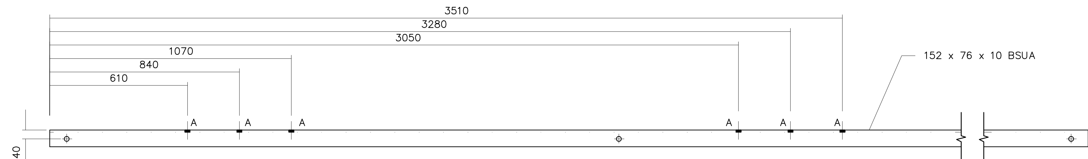
PLAN
